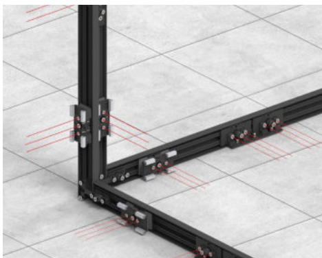
Eckmontage Corner assembly
