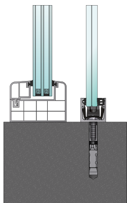
Beton-Rahmen
