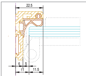
Abb. 8.47: Detail
