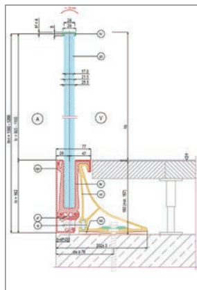
Abb. 8.59: GM RAILING® Solo
