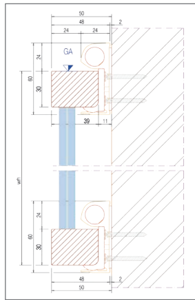
Abb. 8.61: GM WINDOORAIL®
