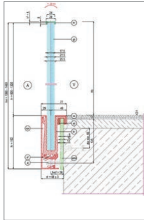
Abb. 8.58: GM RAILING® Side
