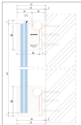
Abb. 8.62: GM WINDOORAIL® Frameless
